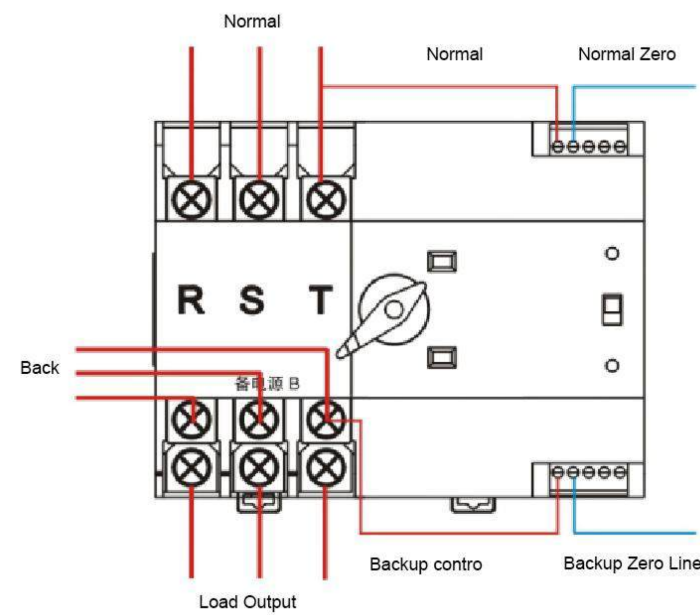
100/3P Wiring Diagram
