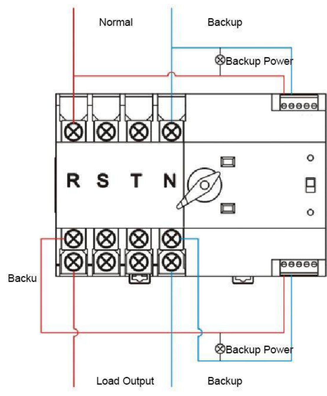
Controller Wiring Diagram
