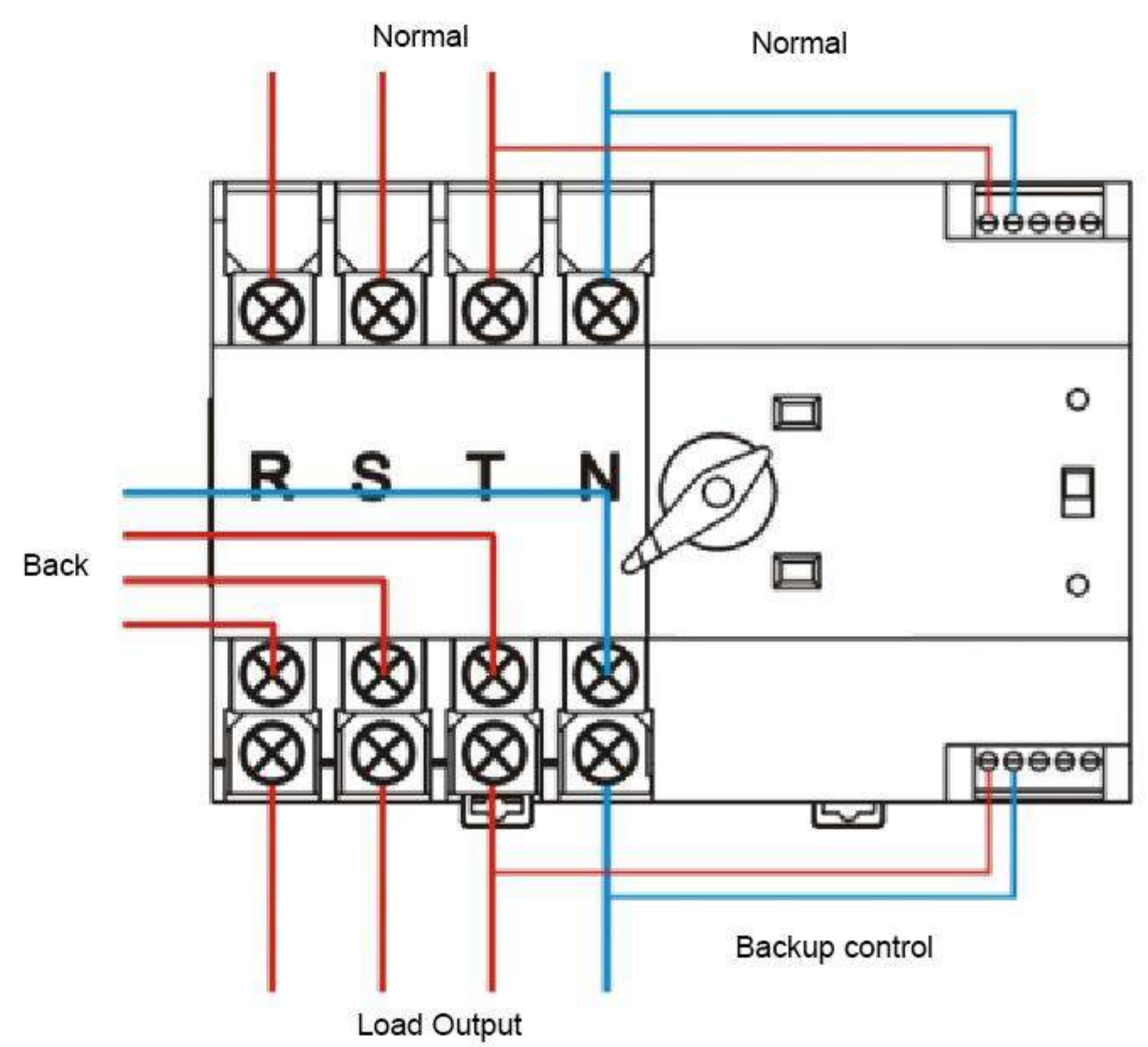
100/4P Wiring Diagram
