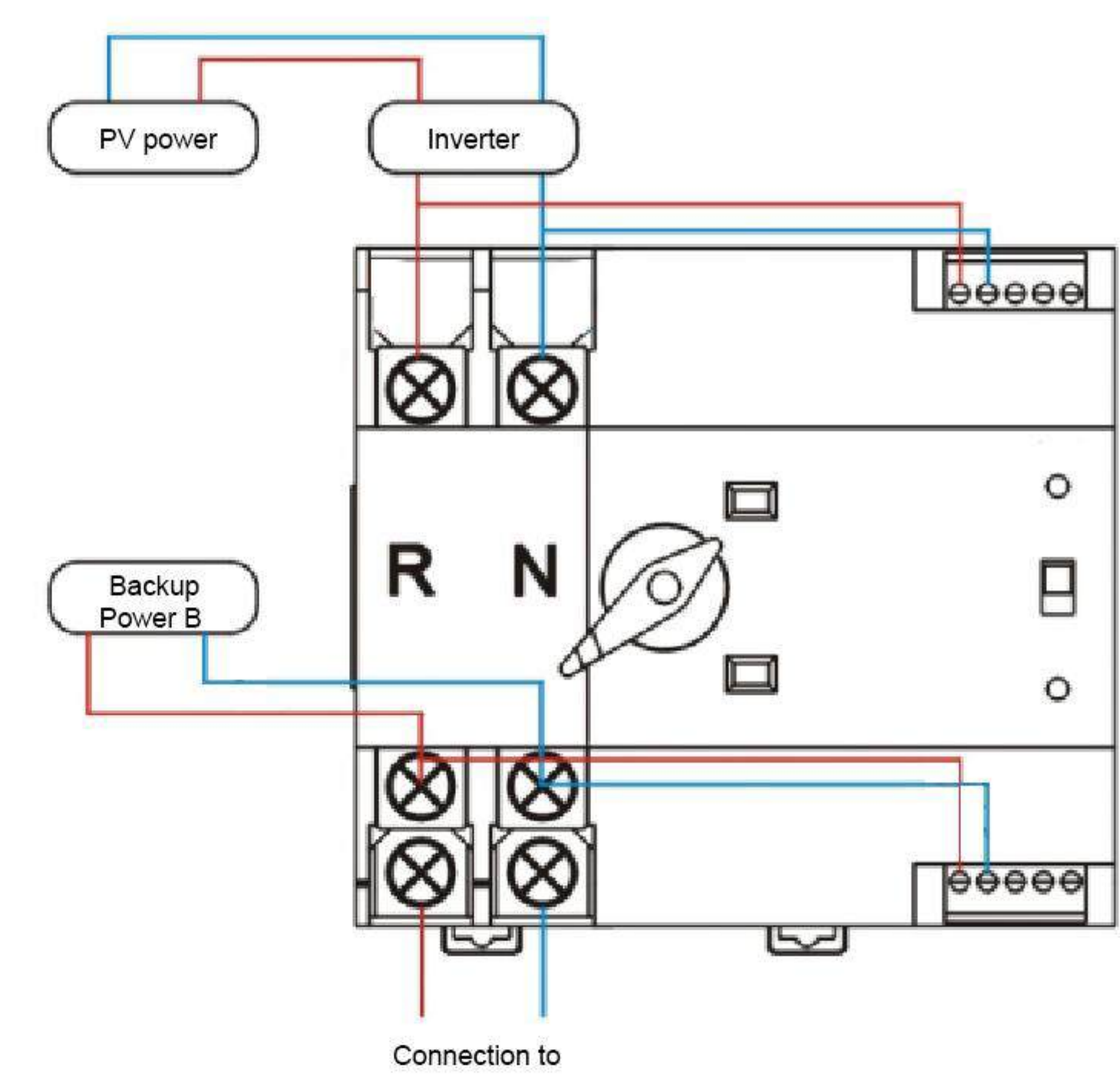
PV inverter-specific wiring
