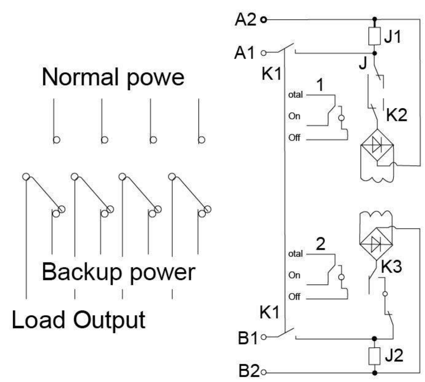
Controller Wiring Diagram
